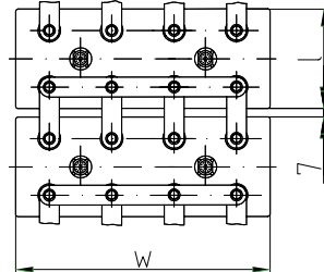
SOL 1110 G – SOL 1245 G (Female thread M10)
