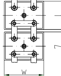
SOL 1385 G - SOL 1525 G (Female thread M10)
